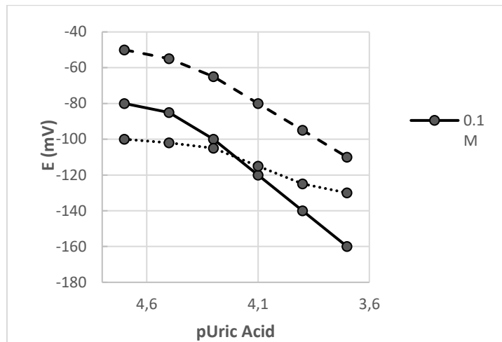
Figure 2. The change of potential with buffer concentration ( 1 \times 10^{-2} M I - ).
