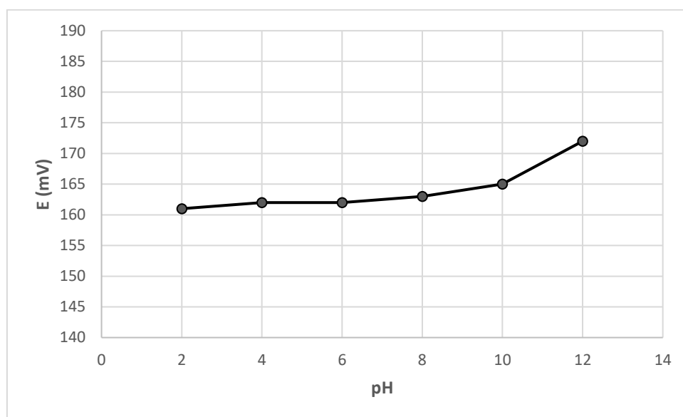
Figure 4. The pH dependence of 20% \text{MoS}_2 , 60% \text{Ag}_2\text{S} and 20% \text{Cu}_2\text{S} electrode in presence of 1 \times 10^{-3} M Mo (VI).
