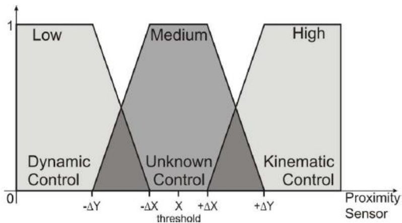
Fig.2 Neutrosophication for the Proximity sensor data
