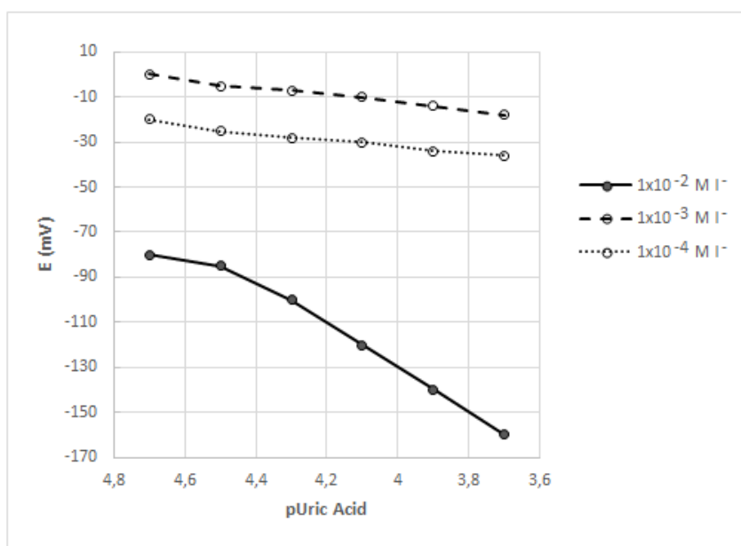
Figure 1. The effect of iodide concentration on the slope of the electrode.
