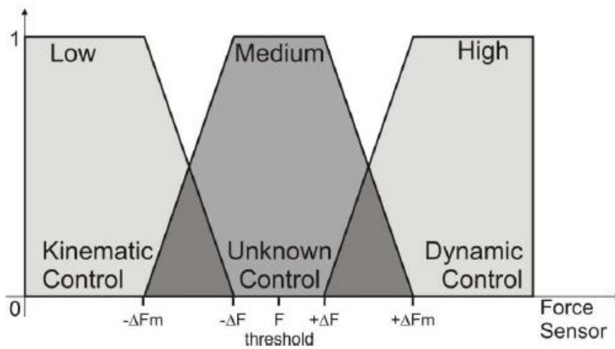
Fig. 3 Neutrosophication for the Force sensor data
