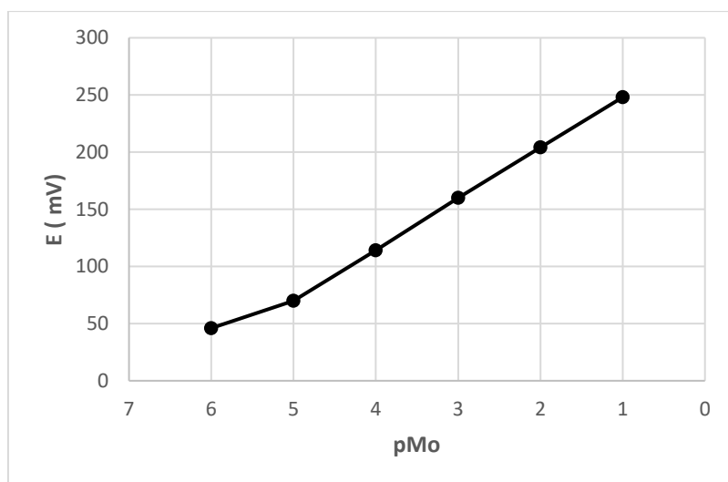
Figure 1. Calibration curve for the newly prepared molybdenum electrode (in 0.1 M \text{NaNO}_3 ).
