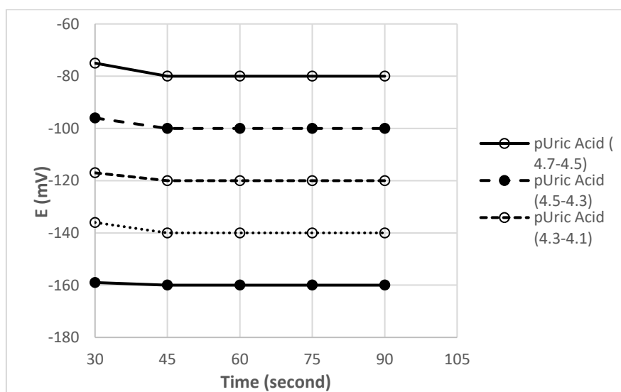
Figure 5. The dependence of response time of the electrode on the change of concentration.
