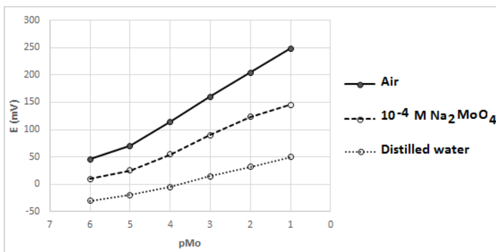
Figure 3. The effect of medium in which the electrode was stored.
