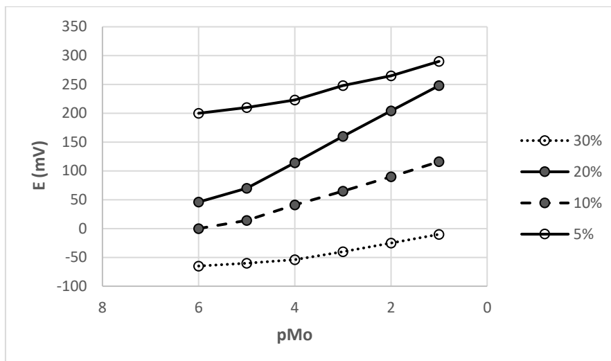
Figure 2. Calibration curves for molybdenum electrodes prepared of different compositions
