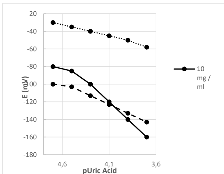
Figure 3. The effect of immobilized enzyme quantity on the slope of the electrode.
