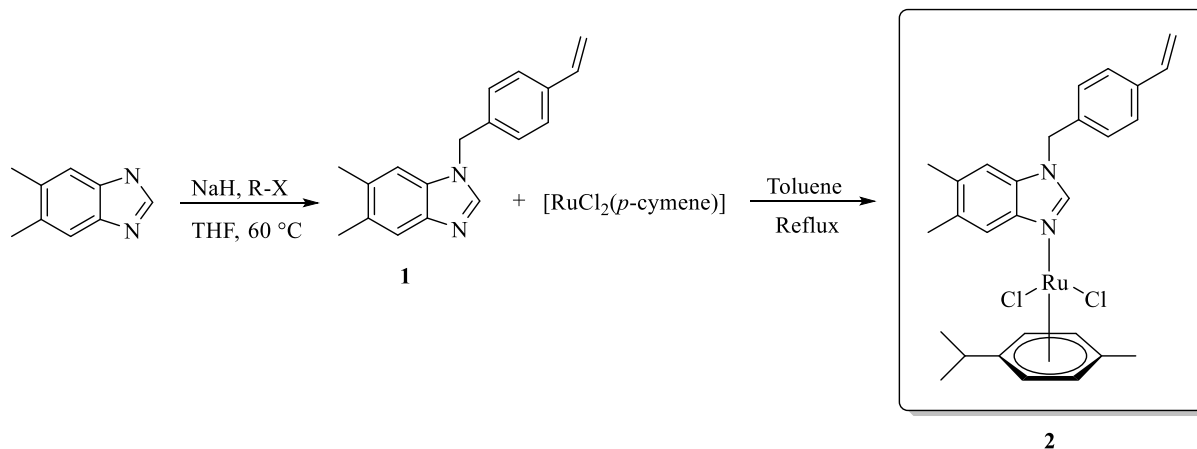
Scheme 1. Synthesis of ruthenium complex
