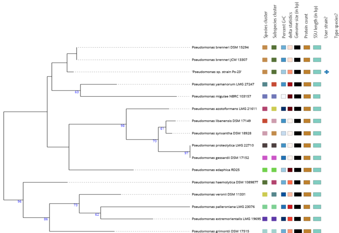
Figure 2. Tree inferred with FastME 2.1.6.1 from GBDP distances calculated from 16S rDNA gene sequences. The branch lengths are scaled in terms of GBDP distance formula d5. The numbers above branches are GBDP pseudo-bootstrap support values > 60 % from 100 replications, with an average branch support of 68.5 %. The tree was rooted at the midpoint.
