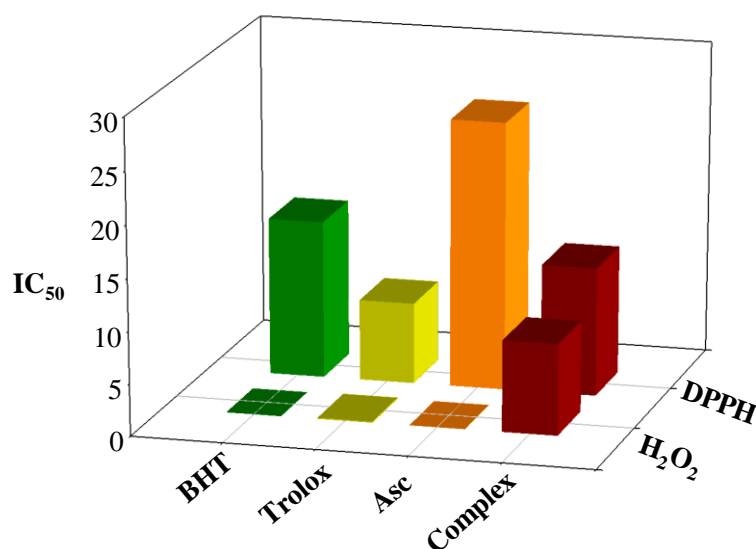
Figure 3 Radical scavenging activities of the complex and comparative antioxidant agents by DPPH and H 2 O 2 assay method
