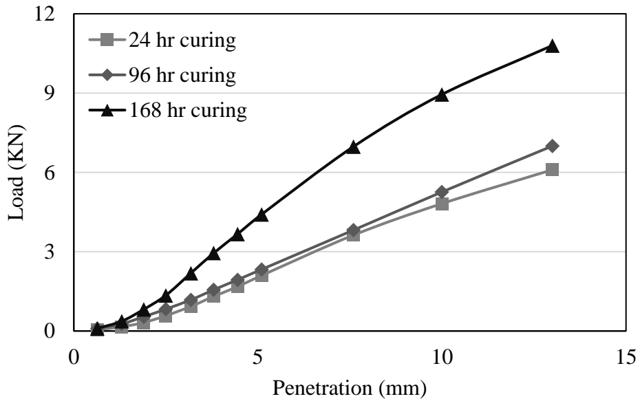
Figure 8: CBR curves of coarse soil with 24, 96, and 168 hour curing time
