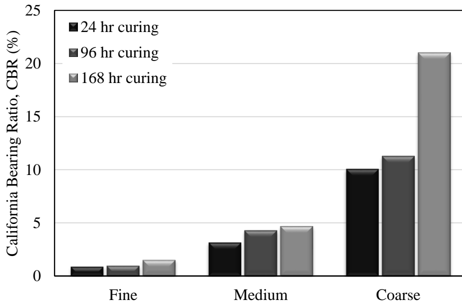
Figure 9: CBR value comparison between fine, medium, and coarse soils
