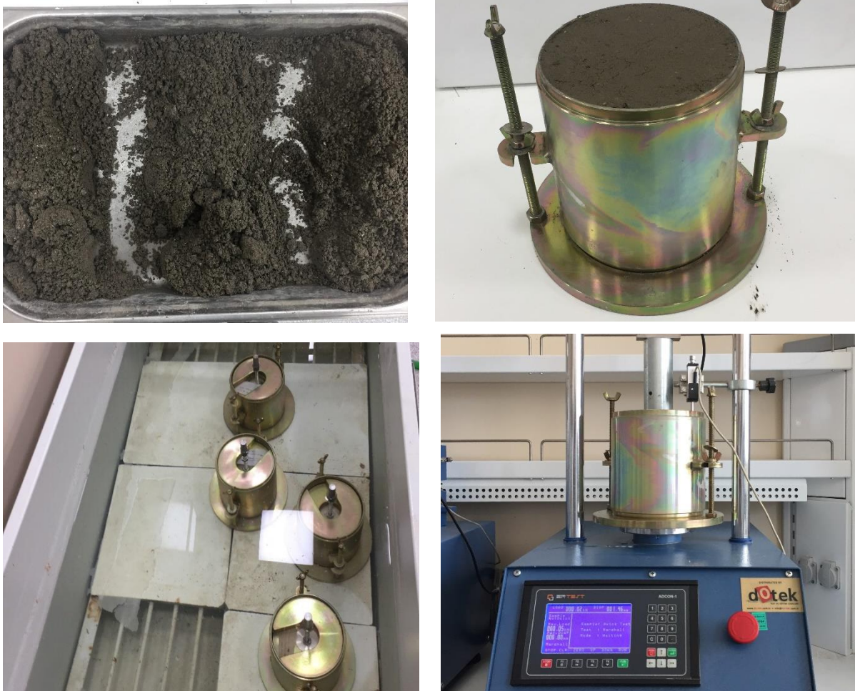
Figure 3: Procedure of CBR test
