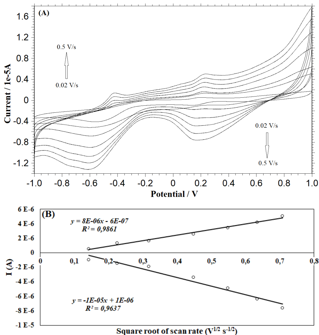
Figure 3. CV of polypyrrole film coated in aqueous phase (50 mM pH 6.5 citrate buffer) in ultra pure water containing 5 mM K_3Fe(CN)_6 at a potential scan ranging between -1 V and +1 V with a scan rate range of 0.02 to 0.5 V/s (inner to outer) (A), plot of redox current values versus the square root of scan rate (B).
