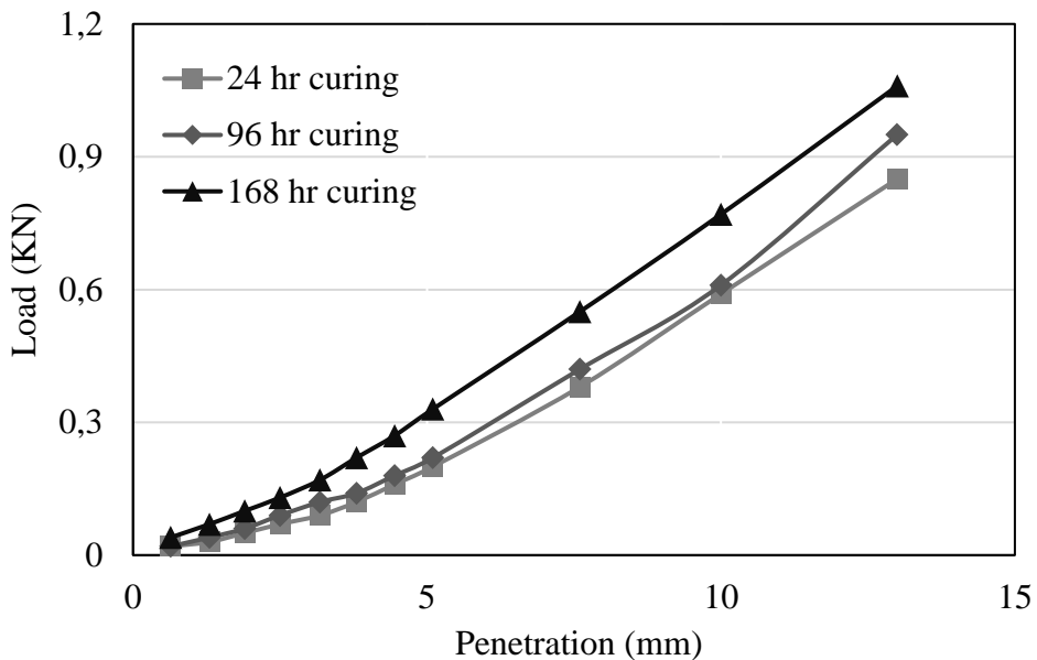
Figure 6: CBR curves of fine soil with 24, 96, and 168 hour curing time
