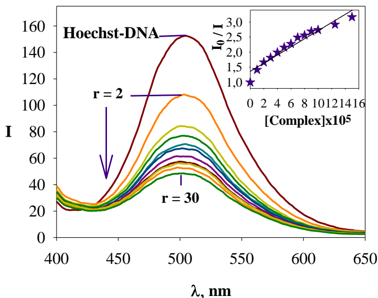
Figure 2. a) Effect of addition of the complex on the emission intensity of the CT-DNA bound EB at different concentrations b) Effect of addition of the complex on the emission intensity of the CT-DNA bound Hoechst 33258 at different concentrations
