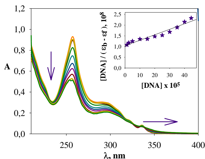
Figure 1. Electronic absorption spectra of the complex upon addition of CT-DNA, Inset: Plot of [DNA]/(\epsilon_b - \epsilon_f) versus [DNA] for the titration of DNA to complex
