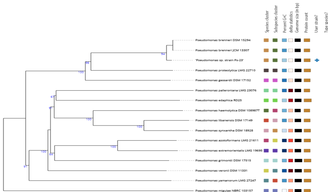
Figure 1. Tree inferred with FastME 2.1.6.1 from GBDP distances calculated from genome sequences. The branch lengths are scaled in terms of GBDP distance formula d5. The numbers above branches are GBDP pseudo-bootstrap support values > 60 % from 100 replications, with an average branch support of 86.5 %. The tree was rooted at the midpoint.
