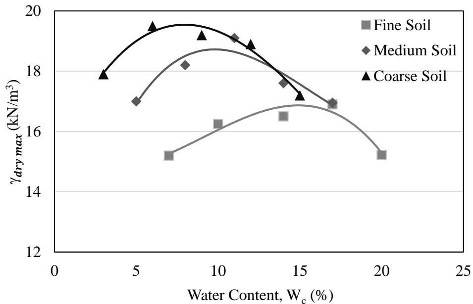
Figure 5: Compaction curves of fine, medium, and coarse samples
