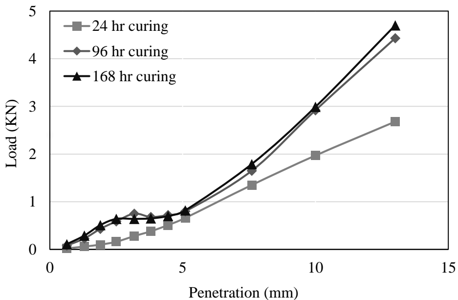
Figure 7: CBR curves of medium soil with 24, 96, and 168 hour curing time
