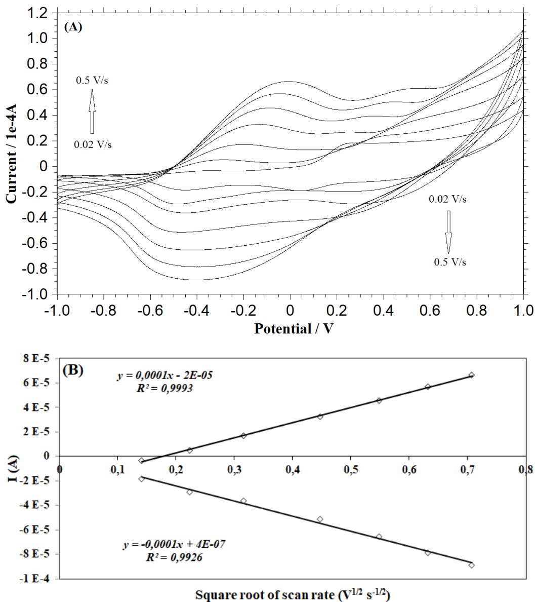
Figure 2. CV of polypyrrole film coated in organic phase (acetonitrile) in ultra pure water containing 5 mM K_3Fe(CN)_6 at a potential scan ranging between -1 V and +1 V with a scan rate range of 0.02 to 0.5 V/s (inner to outer) (A), plot of redox current values versus the square root of scan rate (B).
