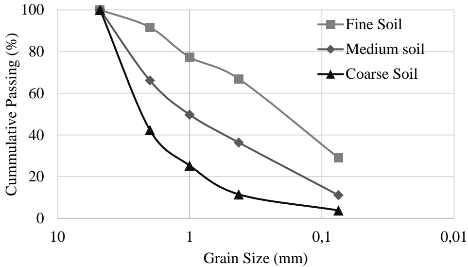
Figure 4: Grain size distribution curves of fine, medium, and coarse samples
