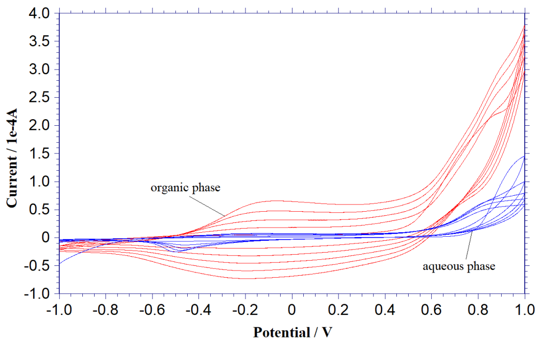
Figure 1. CV of the electrocopolymerization of pyrrole in organic and aqueous phase at a potential scan ranging between -1 and +1 V with the scan rate of 0.1 V/s.
