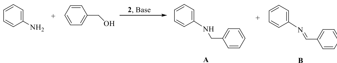
Scheme 2. Optimization studies of N -alkylation reaction of aniline with benzyl alcohol catalyzed by complex 2 .
